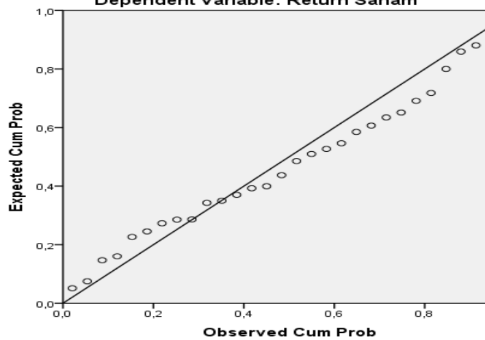
Normal P-P Plot of Regression Standardized Residuals Dependent Variable: Return Saham
